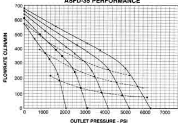
ASFD-35 PERFORMANCE
